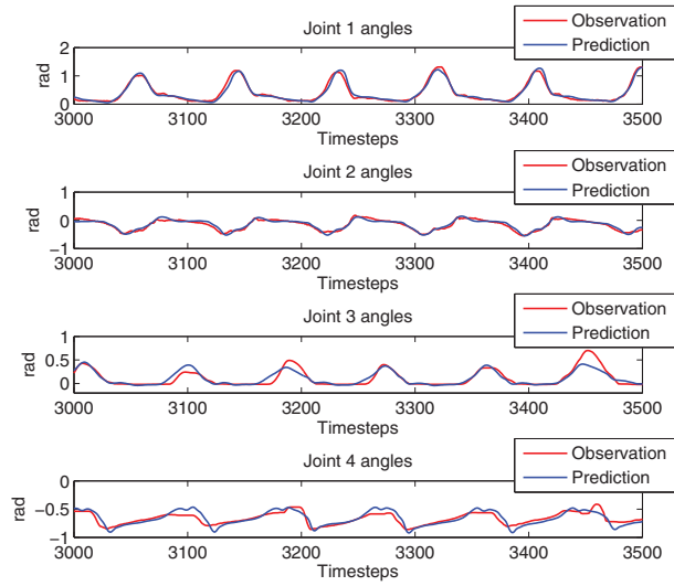
(a) Results of a prediction of the same sequence as shown in Fig. 6b but under cross-subject training data. In this case all joints are observed.
