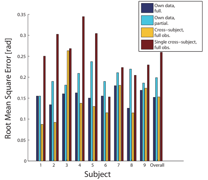
Fig. 5: A comparison-plot of the RMSE results of the approaches with subject-own training data in combination with full and partial observation to two cases of cross-subject training with full observation. In total this figure shows that it is indeed possible to express a person's gait with the generative model constructed from others' data.
