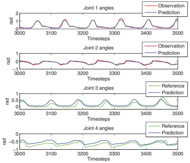
(b) Results of a prediction sequence with subject-own training data under partial observation. Joints 1 and 2 are the observed goniometers, joints 3 and 4 the unobserved exoskeleton-joints.
