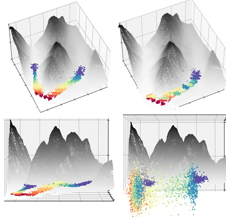
Figure 4: LiDAR Manifold Navigation: CWG before and after guidance (top), CWG vs GSBM (bottom).
