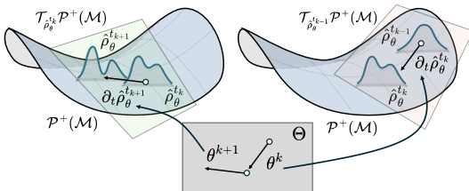
Figure 2: Visualization of the ResNet transformation. Two successive pushforwards \rho_{\theta^{k-1}}^{t_{k-1}} \rightarrow \rho_{\theta^k}^{t_k} \rightarrow \rho_{\theta^{k+1}}^{t_{k+1}} on \mathcal{P}^+(\mathcal{M}) are shown as local updates \partial_t \rho_{\theta^{k-1}}^{t_{k-1}}, \partial_t \rho_{\theta^k}^{t_k} on tangent spaces. Each update is parameterized by \theta^k, \theta^{k+1} \in \Theta , defining local coordinates on \mathcal{TP}^+(\mathcal{M}) . This coordinate system is not unique.
